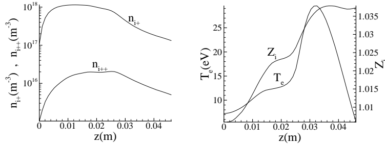
Figure 2. Singly- and doubly-charged ion densities along the channel, n_{i+} and n_{i++} respectively, (left figure) and electron temperature T_e and equivalent ion charge number Z_i along the channel (right figure). All variables are evaluated at the chamber median, r = 0.0425\text{m} .
