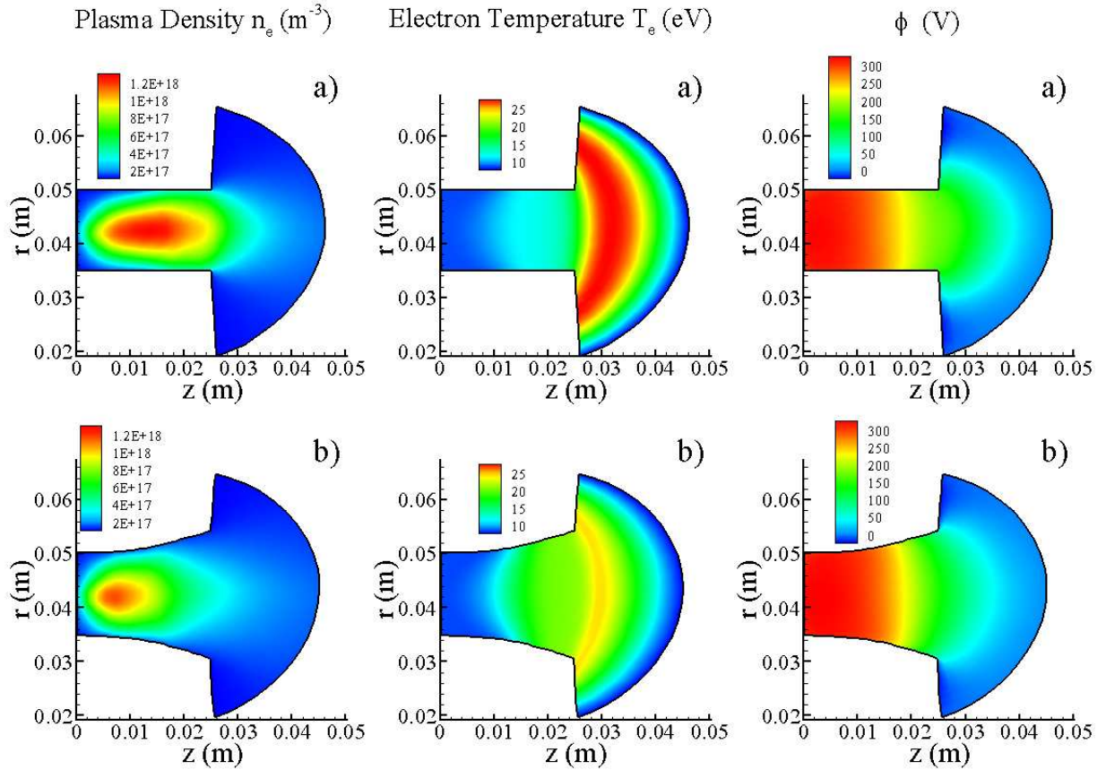
Figure 11. Electron density, n_e(\text{m}^{-3}) , electron temperature, T_e and electric potential, \phi , 2D plots at the initial(a) and final(b) stages of erosion.
