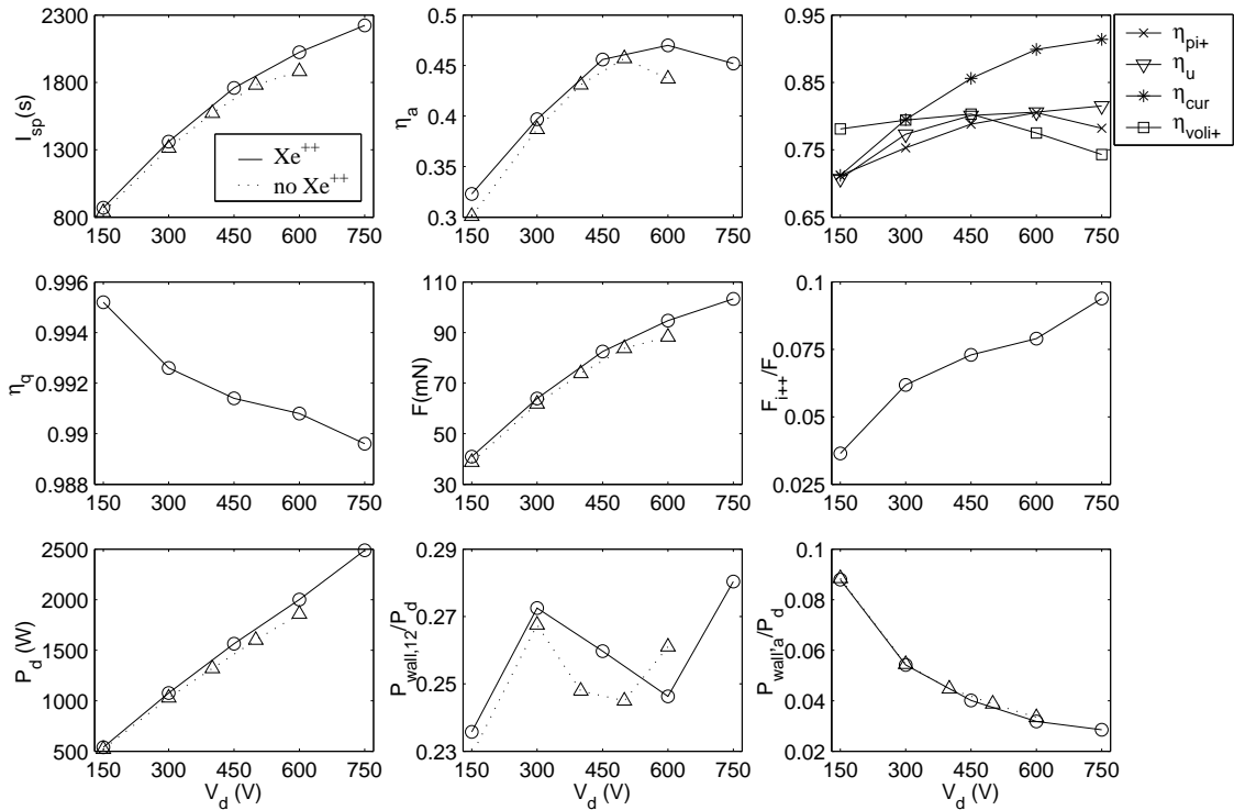
Figure 3. Variation of main operation parameters when varying the discharge potential V_d . P_{wall,12} and P_{wall,a} represent total energy losses to inner and outer walls and to the anode.
