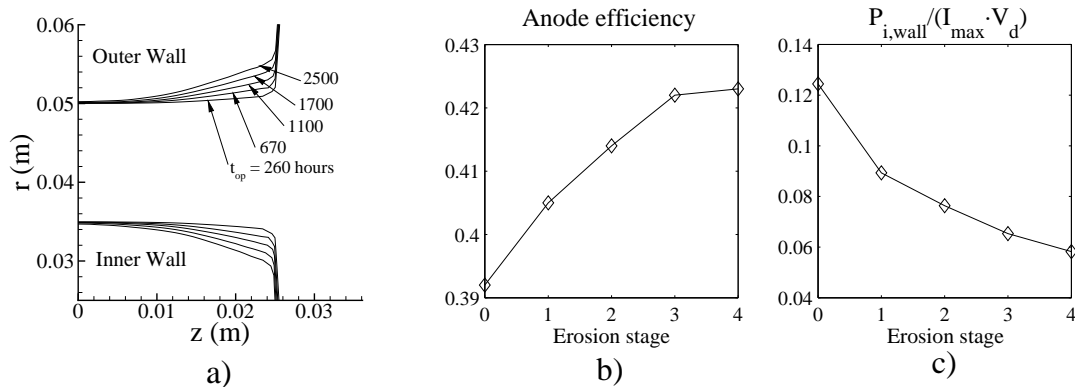
Figure 10. (a) Wall profiles at different erosion stages; t_{op} is the total operation time. (b) Efficiency and (c) total ion energy deposition at the walls after each erosion stage; I_{max} = e\dot{m}_a/m_i .
