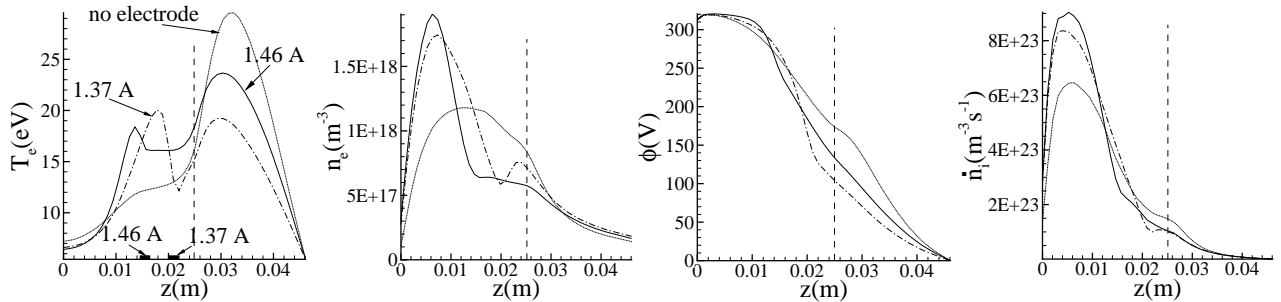
Figure 9. Electron temperature, T_e , electron density, n_e , electric potential, \phi , and total ionization rate, \dot{n}_i , profiles for different location of the electrode and similar currents. Electrode is located on the outer wall at axial positions z=0.021\text{m} and z=0.016\text{m} respectively. In both cases the electrode is 2mm wide. The vertical dashed line represents the thruster exit.
