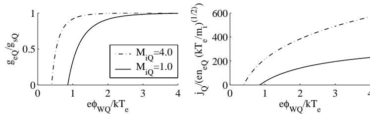
Figure 7. Net electron wall flux to electron emitted flux ratio (left) and non-dimensional wall current(right) as functions of the non-dimensional sheath potential fall for a high-emission electrode.
