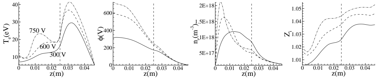
Figure 5. Electron temperature T_e , electric potential \phi , electron density n_e and equivalent charge number Z_i profiles at different discharge voltages ( V_d = 300 V (solid), 600 V (dashed) and 750 V (dashed-dotted)). All variables are evaluated at the outer wall ( r = 0.0425 m). The vertical dashed line represents the thruster exit.
