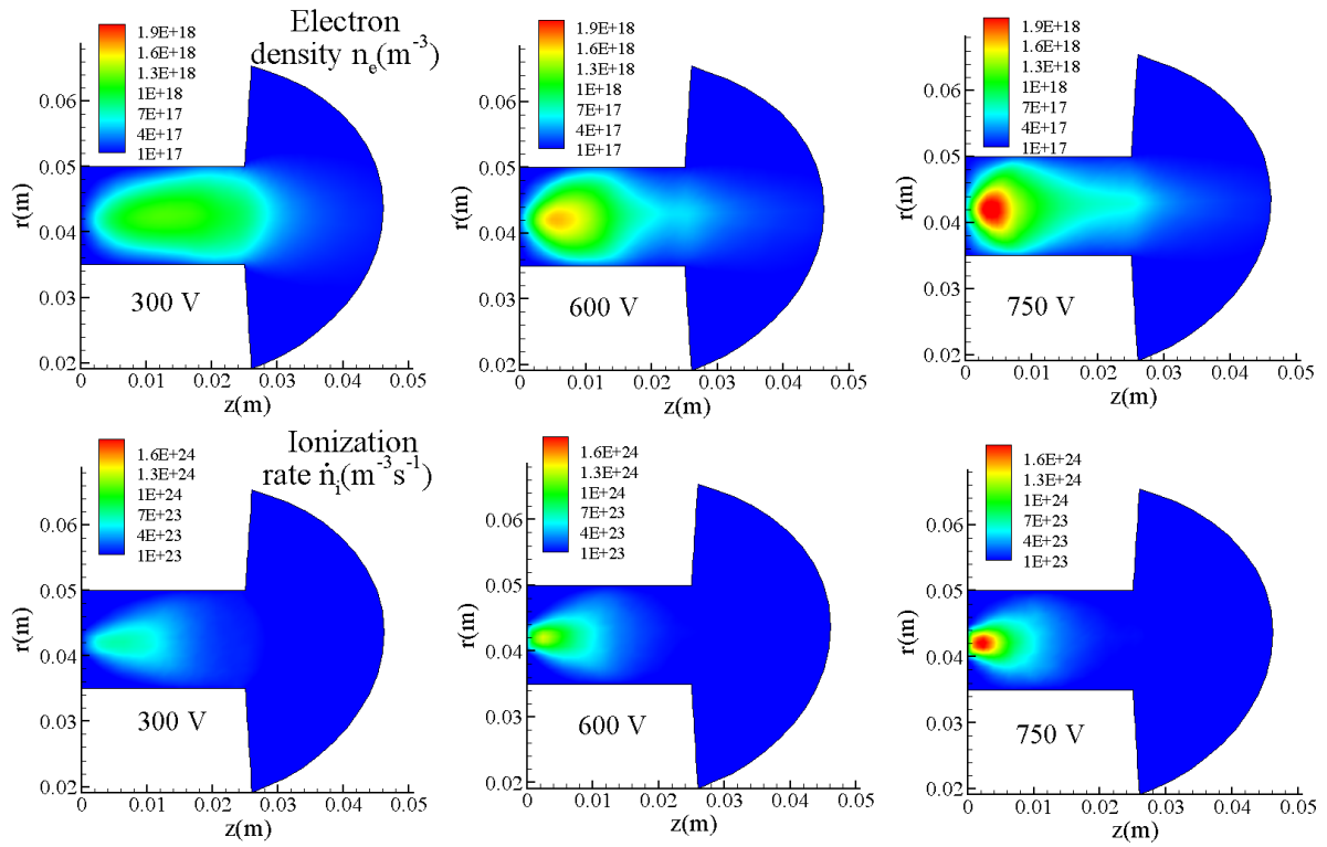
Figure 4. Electron density, n_e (upper figures), and total ionization rate, \dot{n}_i (lower figures) at V_d = 300 V, 600 V and 750 V, for the previous parametric variation.
