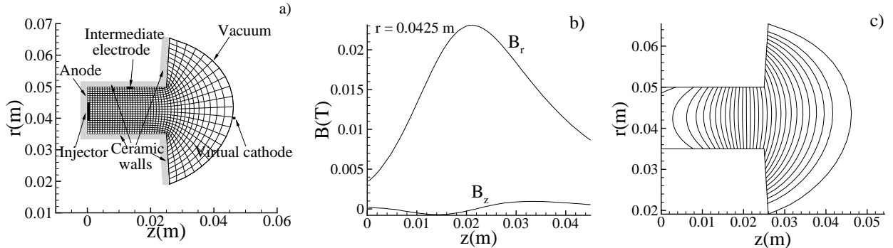
Figure 1. Elements of the simulated SPT-100 type simulated thruster and PIC-mesh(a), reference magnetic field at the chamber median, B_r and B_z are the radial and axial components respectively(b) and magnetic streamsurfaces used in the electron-mesh(c).
