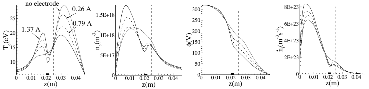
Figure 8. Electron temperature, T_e , electron density, n_e , electric potential, \phi , and total ionization rate, \dot{n}_i , profiles for different currents through the electrode. The electrode is 2mm wide and is located on the outer wall at axial position z=21\text{mm} . The vertical dashed line represents the thruster exit.
