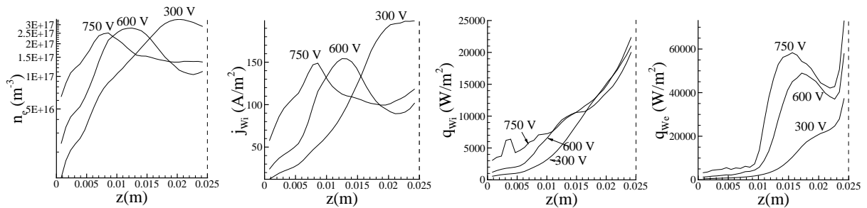
Figure 6. Electron density, n_e , ion current to wall, j_{wi} , ion energy flux to wall, q_{wi} , and electron energy flux to wall, q_{we} for V_d = 300 V, 600 V and 750 V. All variables are evaluated at the outer wall ( r = 0.05 m). The vertical dashed line represents the thruster exit.
